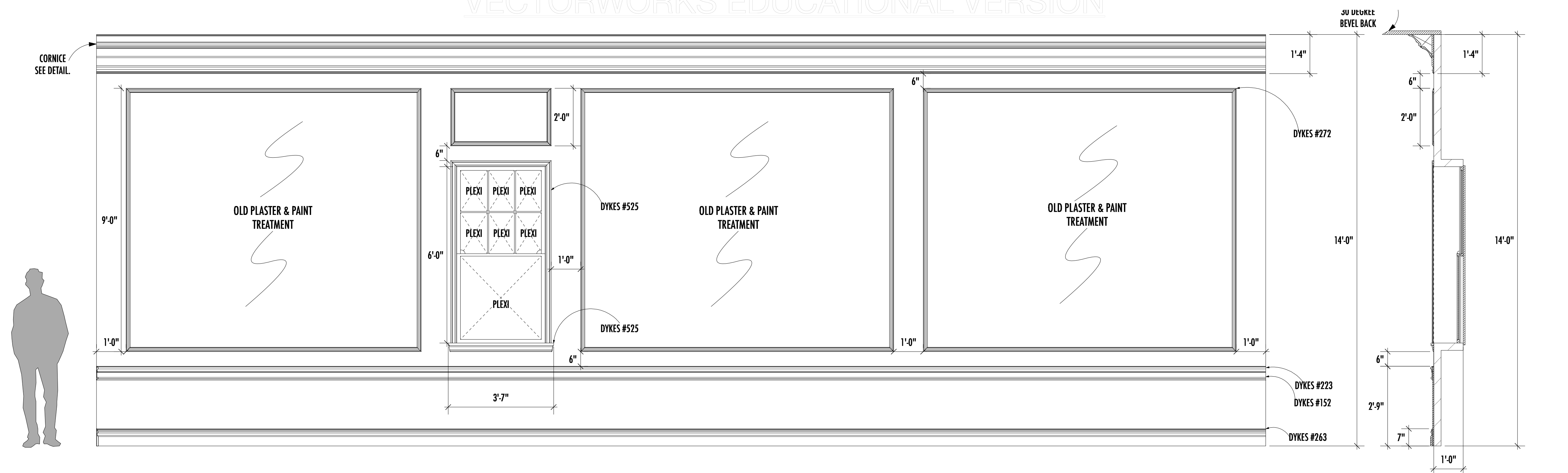
FRONT ELEVATION-WALL B Scale: 1/2" = 1'-0"
