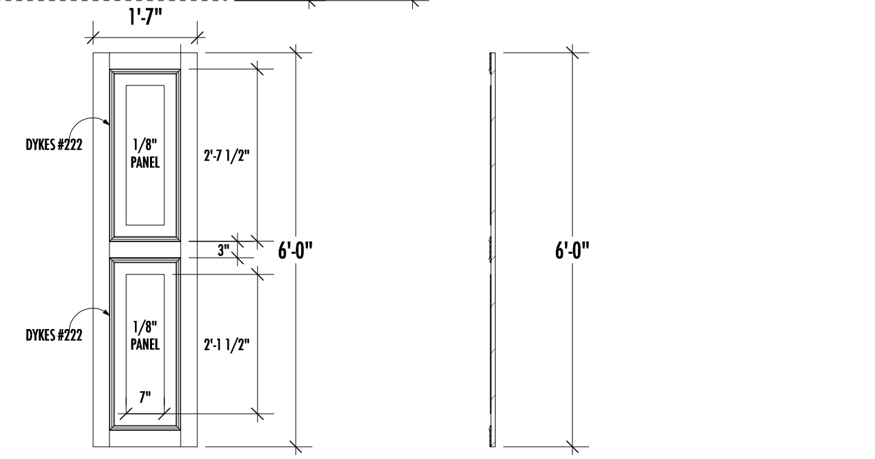
SHUTTER-FRONT ELEVATION Scale: 1/2" = 1'-0"
