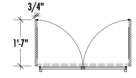
SHUTTER-PLAN VIEW Scale: 1/2" = 1'-0"
